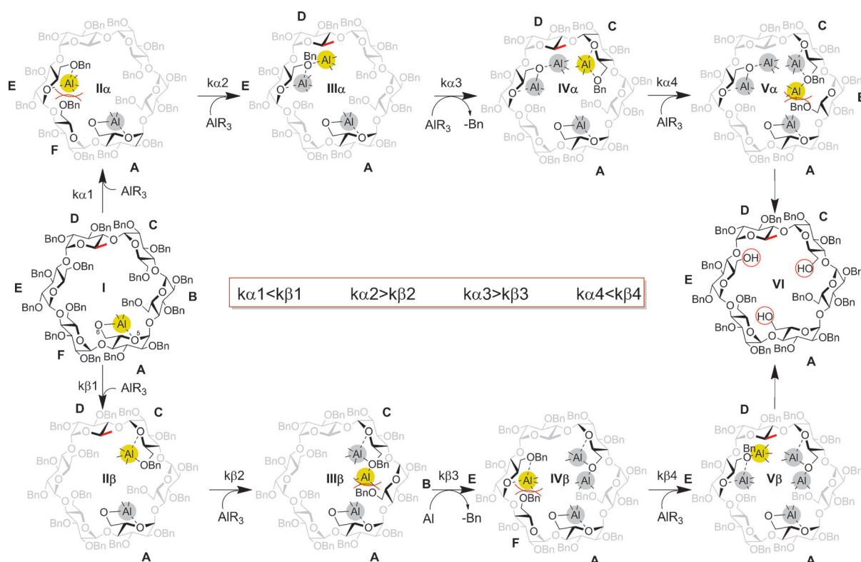
Scheme 3. Mechanistic proposal.
